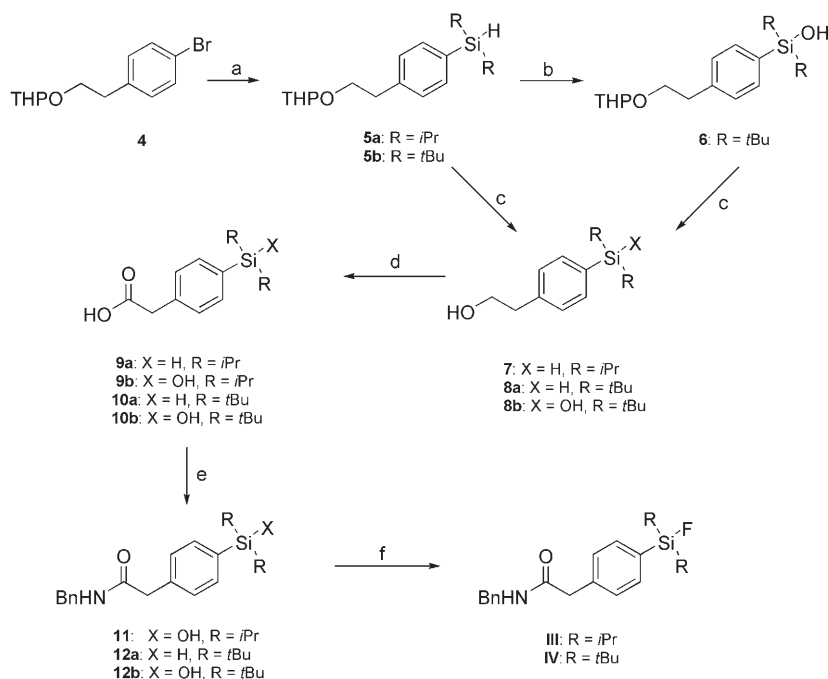
Scheme 2. Synthesis of silane derivatives with aryl linkers. a) 5a : n BuLi, i PrMgBr, THF, i Pr 2 SiClH, 97%; 5b : n BuLi, THF, t Bu 2 SiClH, 74%; b) 6 : KOH, EtOH, 71%; c) 7 : p TsOH, EtOH, 93%; 8a and 8b : TsOH, EtOH; d) 9a : Jones reagent, acetone, 69%; 9b : Pd/C, H 2 O, CCl 4 from 9a 69%; 10a : from 5b , 1. p TsOH, EtOH, 2. Jones reagent, acetone, overall yield 80%; 10b : from 6 , 1. TsOH, EtOH, 2. Jones reagent, acetone, overall yield 77%; e) 11 : starting with 9a , 1. NHS, EDC·HCl, CH 2 Cl 2 , 83%; 2. Pd/C, H 2 O, CCl 4 , 78%; 3. BnNH 2 , CH 2 Cl 2 , 76%; 12a and 12b : EDC·HCl, BnNH 2 , CH 2 Cl 2 , 66% for 12a and 76% for 12b ; f) KF/crypt-222, AcOH, THF, 81% for compound III , 98% for compound IV from 12a . THP = tetrahydropyranyl, Bn = benzyl, Ts = toluenesulfonyl.
