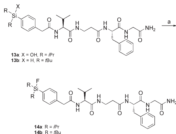
Scheme 4. ^{18}\text{F} -radiolabeling of silicon tetrapeptides. a) \text{K}[^{18}\text{F}]\text{F} , 5 mg crypt-222, 1 mg \text{K}_2\text{CO}_3 , 3 \mu\text{L} AcOH, 1 mg 13a in 0.3 mL DMSO, 15 min, 90 °C, 53% conversion for 14a ; \text{K}[^{18}\text{F}]\text{F} , 5 mg crypt-222, 1 mg \text{K}_2\text{CO}_3 , 2 mg 13b in 0.3 mL DMSO, 15 min, 65 °C, 45% conversion for 14b .
