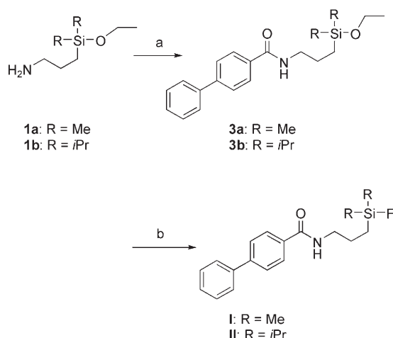
Scheme 1. Synthesis of silane derivatives with alkyl linkers. a) Biphenyl-4-carbonyl chloride ( 2 ), NEt 3 , dioxane, RT, 1 h for 3a , 61%; 1.5 h for 3b , 55%; b) BF 3 ·OEt 2 , Et 2 O, reflux, 15 min for compound I , 63%; 30 min for compound II , 97%.
